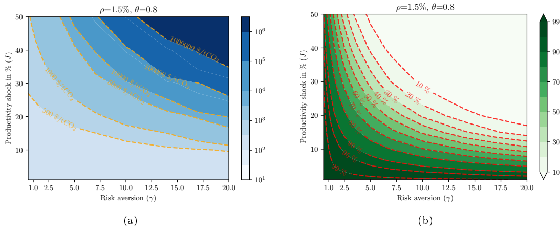
Fig. 3 Comparison of the Social Cost of Carbon to a risk-free SCC under expected damages for Epstein-Zin preferences: Heatmap of the Social Cost of Carbon (panel a., in US$2005) and the share of its value that can be explained by expected damages (panel b., ratio SCC^{ed}/SCC ). The ratio decreases with risk aversion and with the magnitude of the shock, but remains above 90% for productivity shocks lower than 10%, unless risk aversion is greater than 10.
